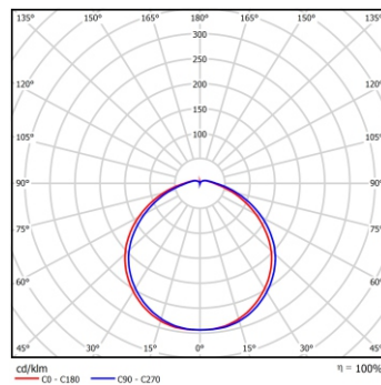
ToLEDo High Bay 100W
