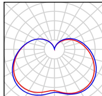
ToLEDo High Bay 40W
